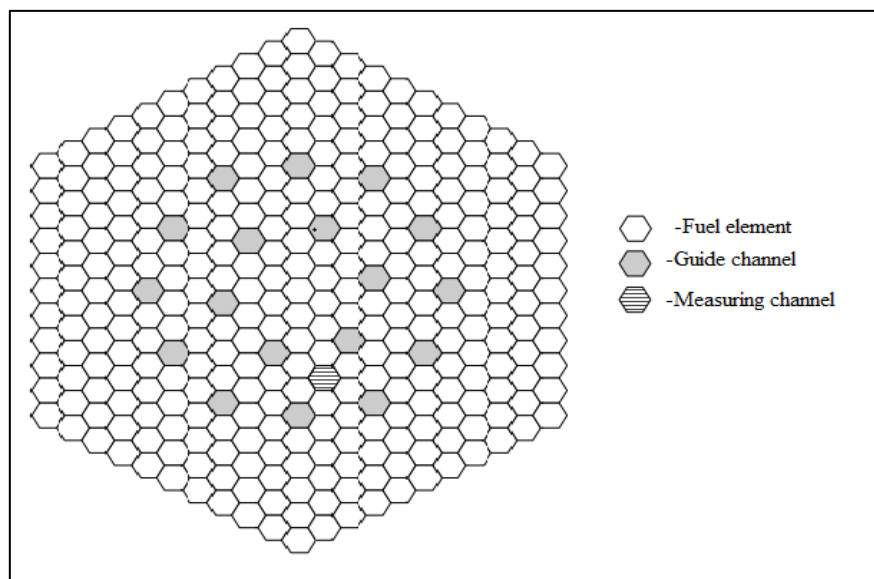
Figure 1– Cartogram fuel assemblies Z13, Z40, and Z49 of the reactor VVER-1200
